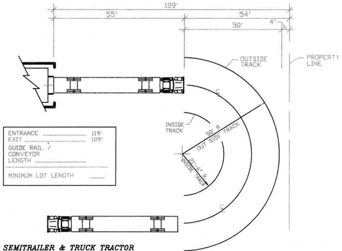
SEMITRAILER & TRUCK TRACTOR EXIT SPECIFICATIONS 35' TO 55' VEHICLES
